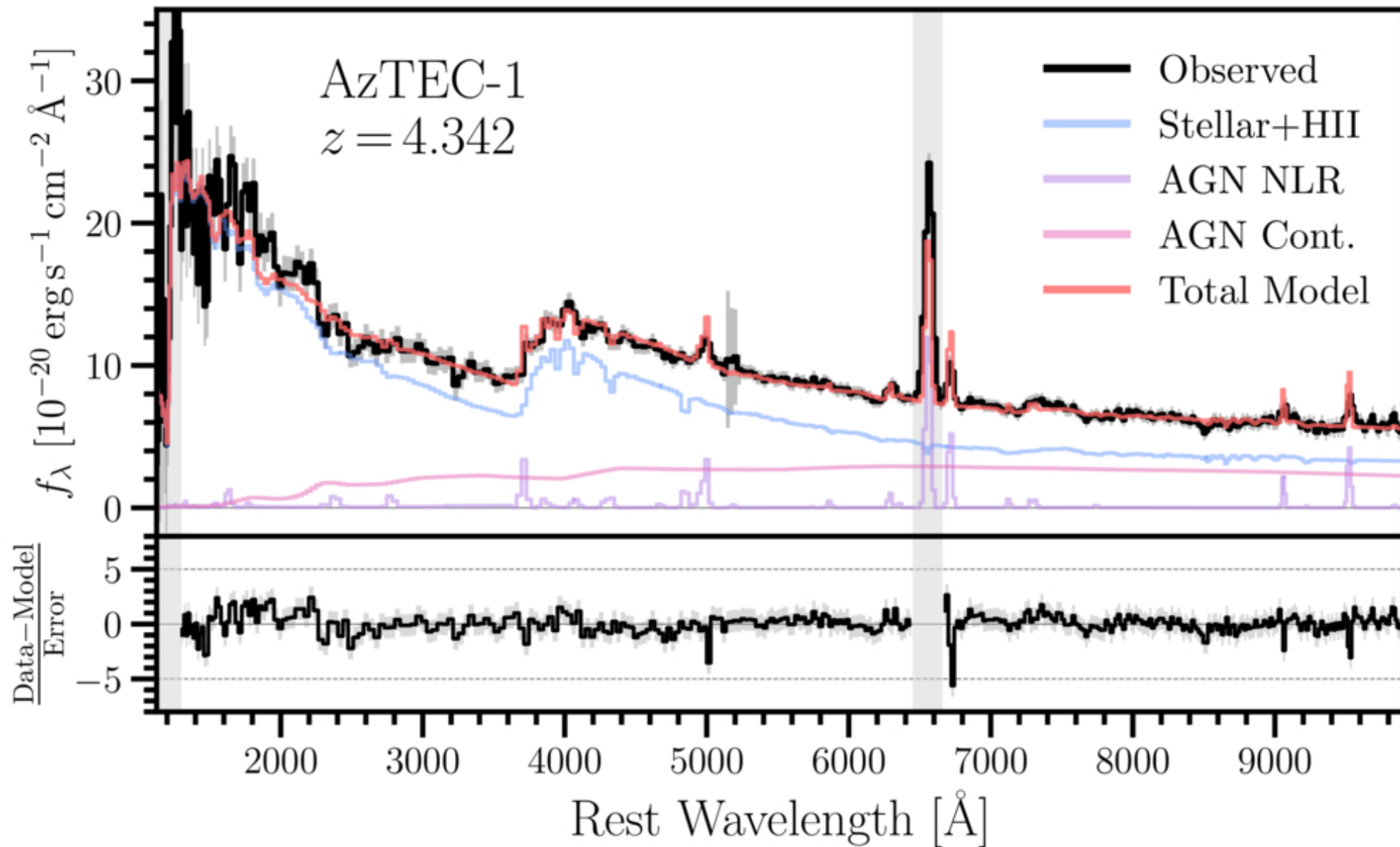
Figure 7. from Jed McKinney et al 2026 Astrophys. J. Lett. 1011 doi:10.3847/2041-8213/aea0cd https://dx.doi.org/10.3847/2041-8213/aea0cd © 2026. The Author(s). Published by the American Astronomical Society.
