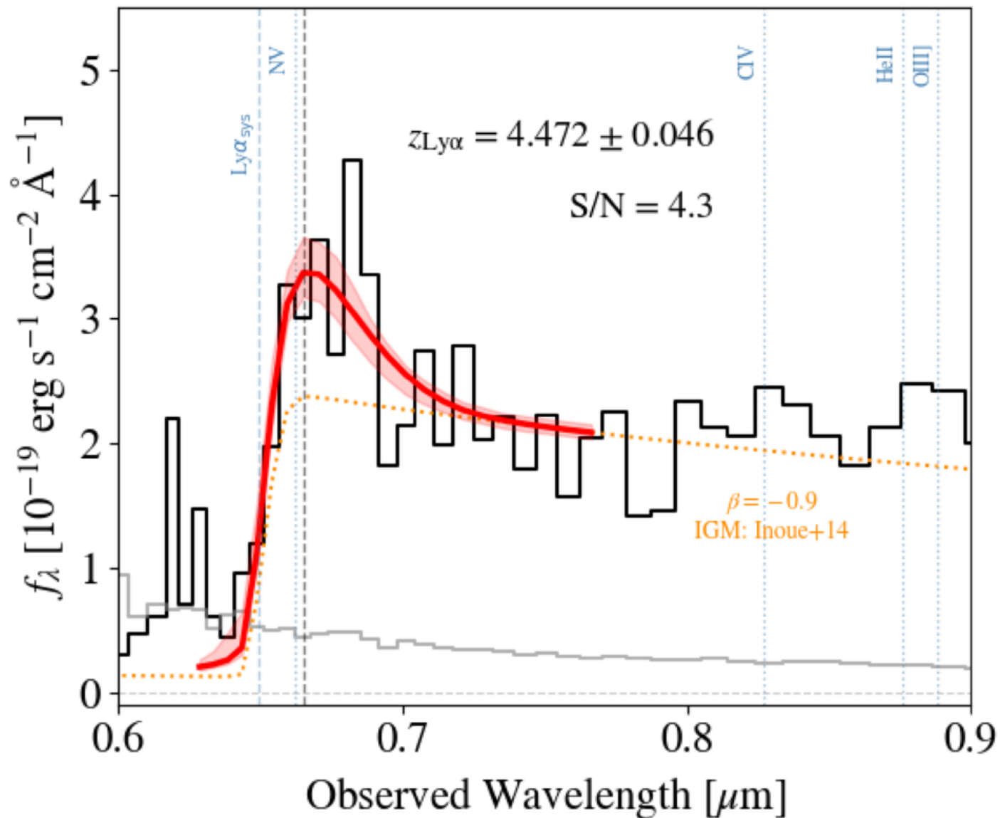
Figure 6. from Jed McKinney et al 2026 Astrophys. J. Lett. 1011 doi:10.3847/2041-8213/aea0cd https://dx.doi.org/10.3847/2041-8213/aea0cd © 2026. The Author(s). Published by the American Astronomical Society.
