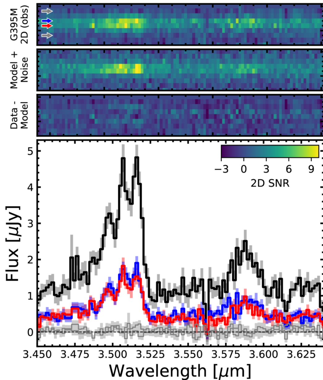
Figure 5. from Jed McKinney et al 2026 Astrophys. J. Lett. 1011 doi:10.3847/2041-8213/aea0cd https://dx.doi.org/10.3847/2041-8213/aea0cd © 2026. The Author(s). Published by the American Astronomical Society.
