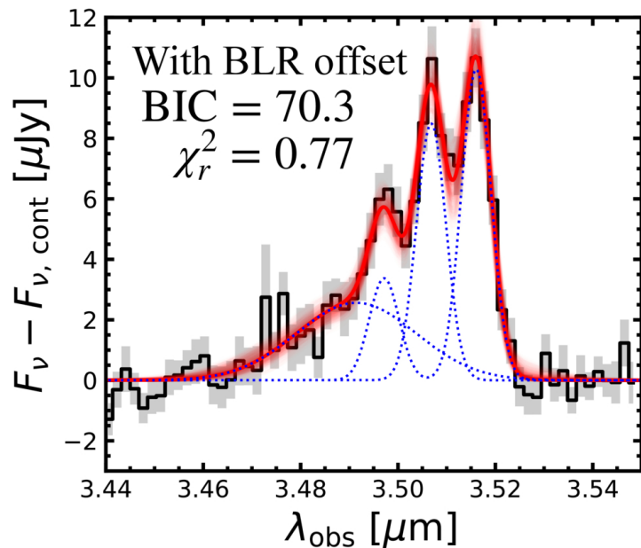
Figure 4. from Jed McKinney et al 2026 Astrophys. J. Lett. 1011 doi:10.3847/2041-8213/aea0cd https://dx.doi.org/10.3847/2041-8213/aea0cd © 2026. The Author(s). Published by the American Astronomical Society.
