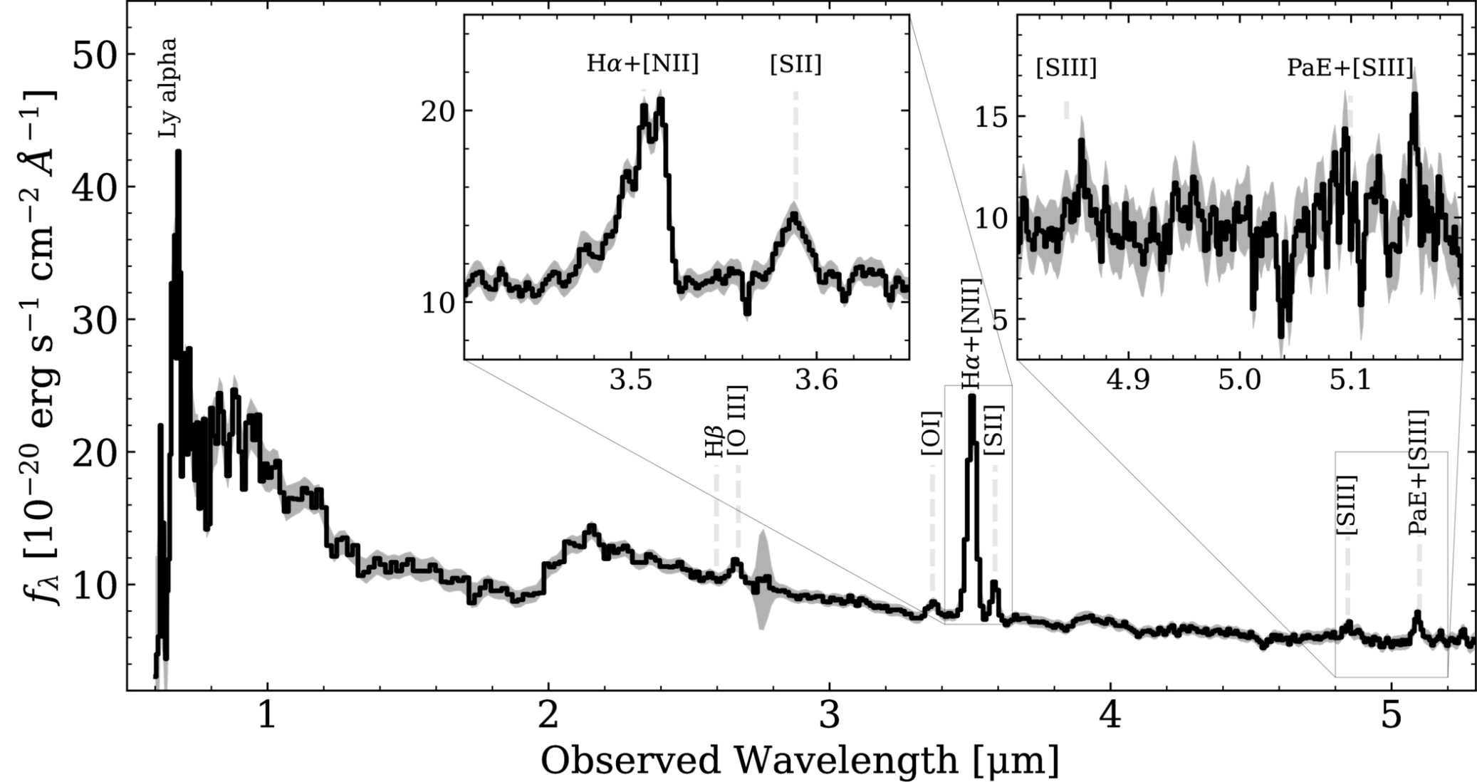
Figure 3. from Jed McKinney et al 2026 Astrophys. J. Lett. 1011 doi:10.3847/2041-8213/aea0cd https://dx.doi.org/10.3847/2041-8213/aea0cd © 2026. The Author(s). Published by the American Astronomical Society.
