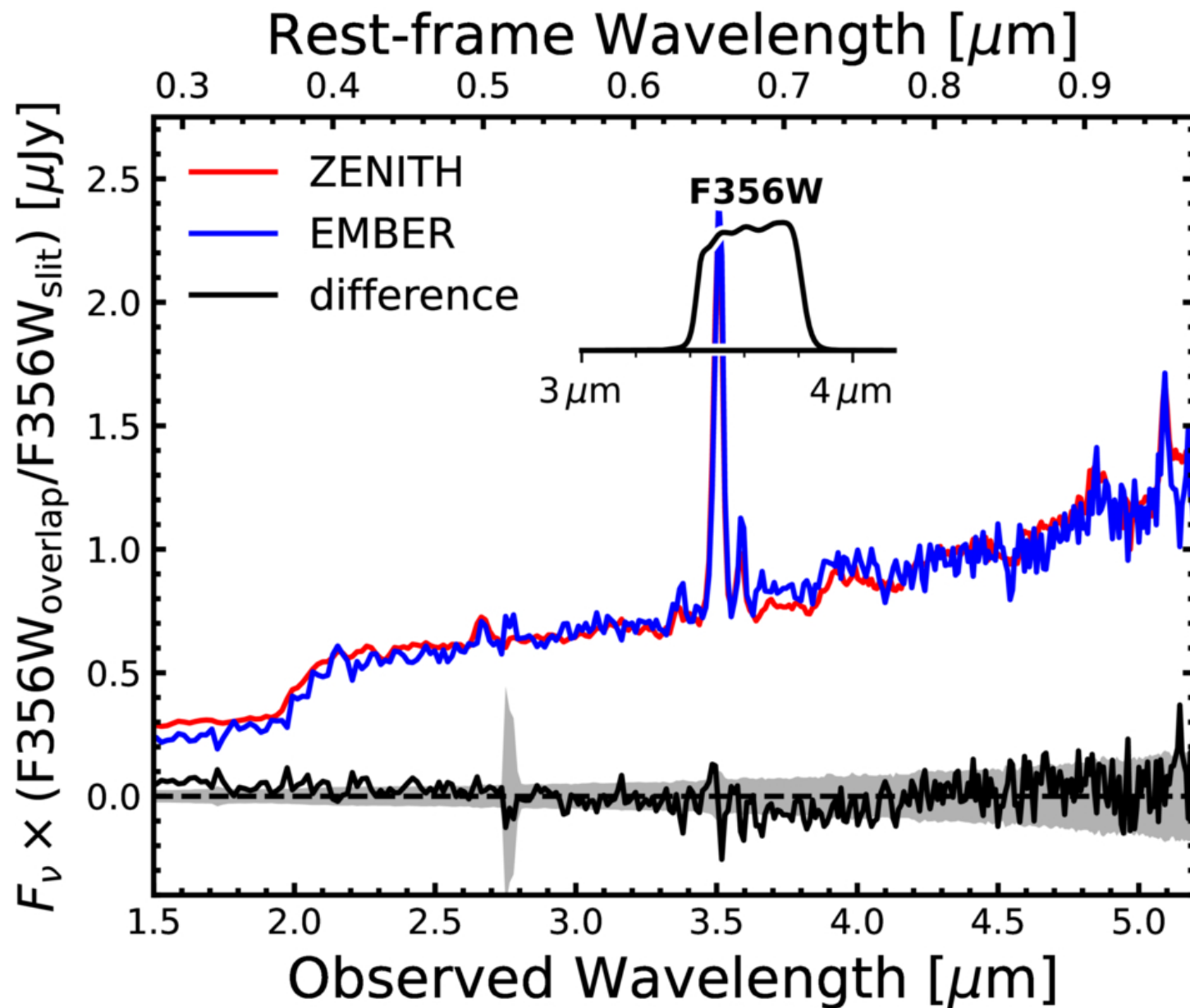
Figure 2. from Jed McKinney et al 2026 Astrophys. J. Lett. 1011 doi:10.3847/2041-8213/aea0cd https://dx.doi.org/10.3847/2041-8213/aea0cd © 2026. The Author(s). Published by the American Astronomical Society.
