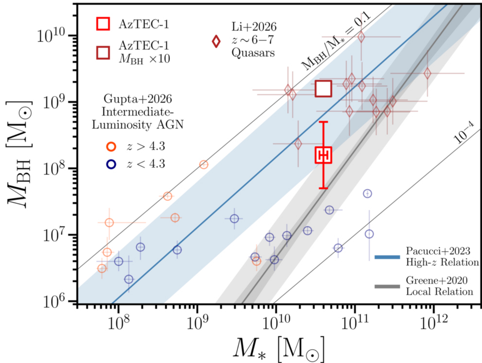
Figure 12. from Jed McKinney et al 2026 Astrophys. J. Lett. 1011 doi:10.3847/2041-8213/aea0cd https://dx.doi.org/10.3847/2041-8213/aea0cd © 2026. The Author(s). Published by the American Astronomical Society.
