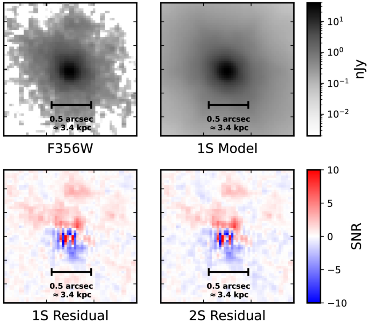
Figure 10. from Jed McKinney et al 2026 Astrophys. J. Lett. 1011 doi:10.3847/2041-8213/aea0cd https://dx.doi.org/10.3847/2041-8213/aea0cd © 2026. The Author(s). Published by the American Astronomical Society.
