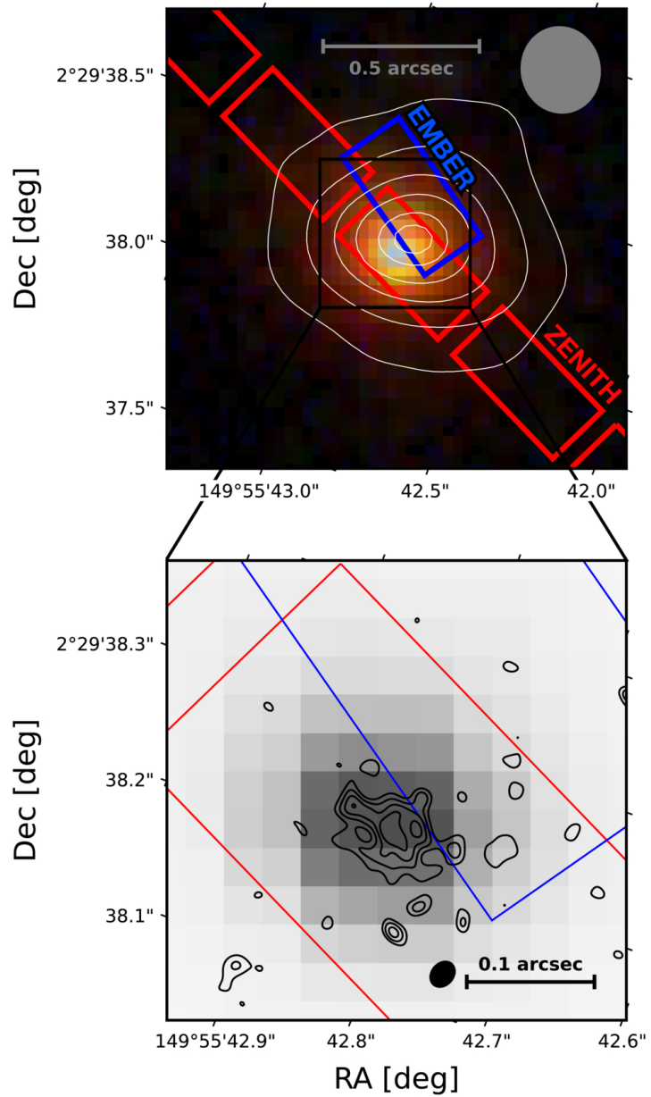
Figure 1. from Jed McKinney et al 2026 Astrophys. J. Lett. 1011 doi:10.3847/2041-8213/aea0cd https://dx.doi.org/10.3847/2041-8213/aea0cd © 2026. The Author(s). Published by the American Astronomical Society.
