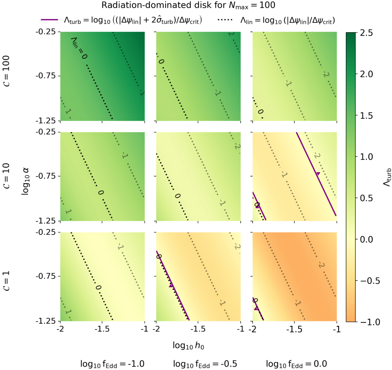
Figure 3. from Mudit Garg et al 2026 Astrophys. J. Lett. 1009 doi:10.3847/2041-8213/aea0ca https://dx.doi.org/10.3847/2041-8213/aea0ca © 2026. The Author(s). Published by the American Astronomical Society.
