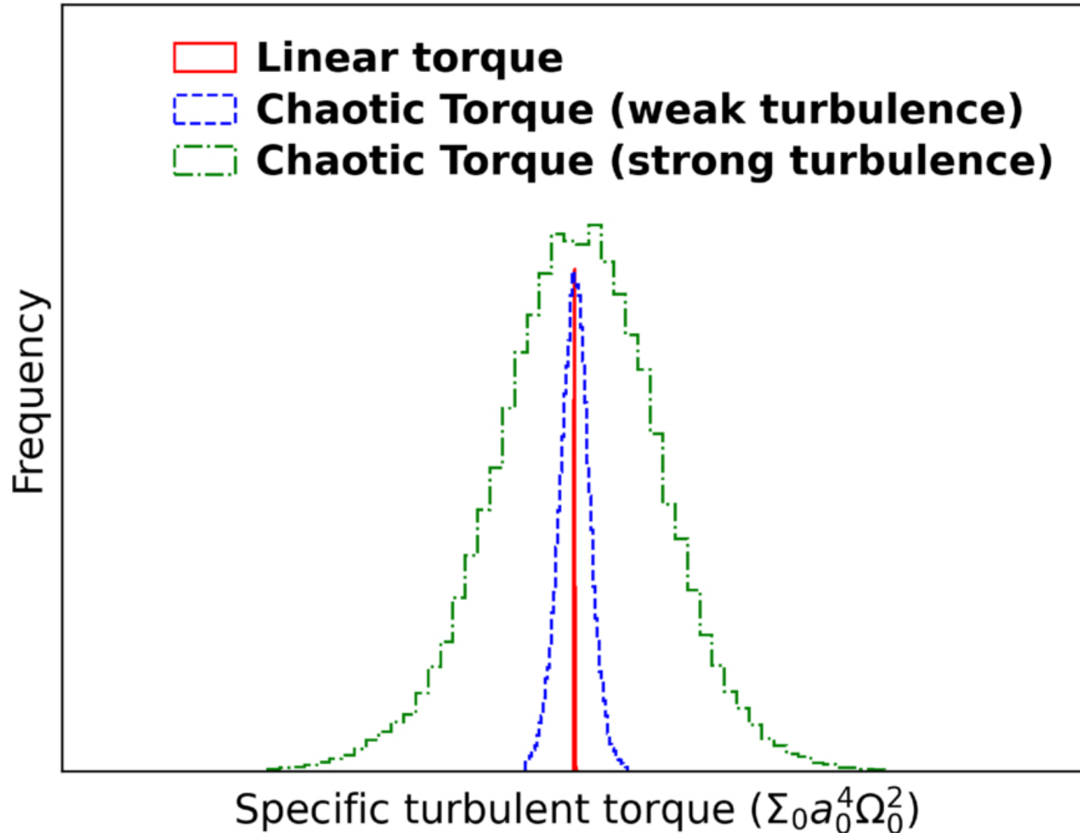
Figure 1. from Mudit Garg et al 2026 Astrophys. J. Lett. 1009 doi:10.3847/2041-8213/aea0ca https://dx.doi.org/10.3847/2041-8213/aea0ca © 2026. The Author(s). Published by the American Astronomical Society.
