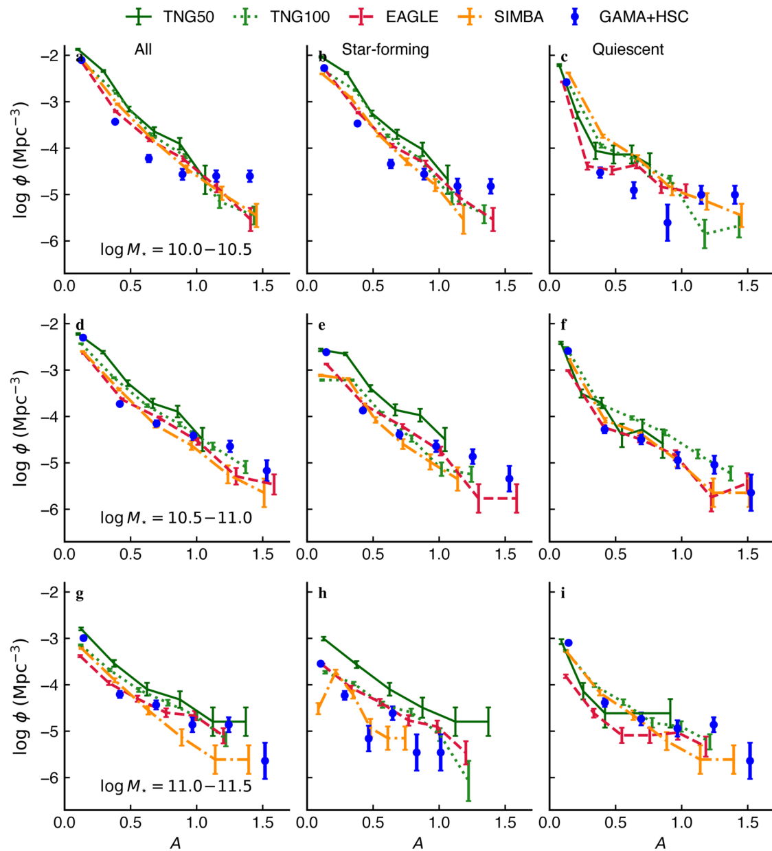
Figure 5. from Hassen M. Yesuf et al 2026 Astrophys. J. Lett. 1009 doi:10.3847/2041-8213/aea0c6 https://dx.doi.org/10.3847/2041-8213/aea0c6
