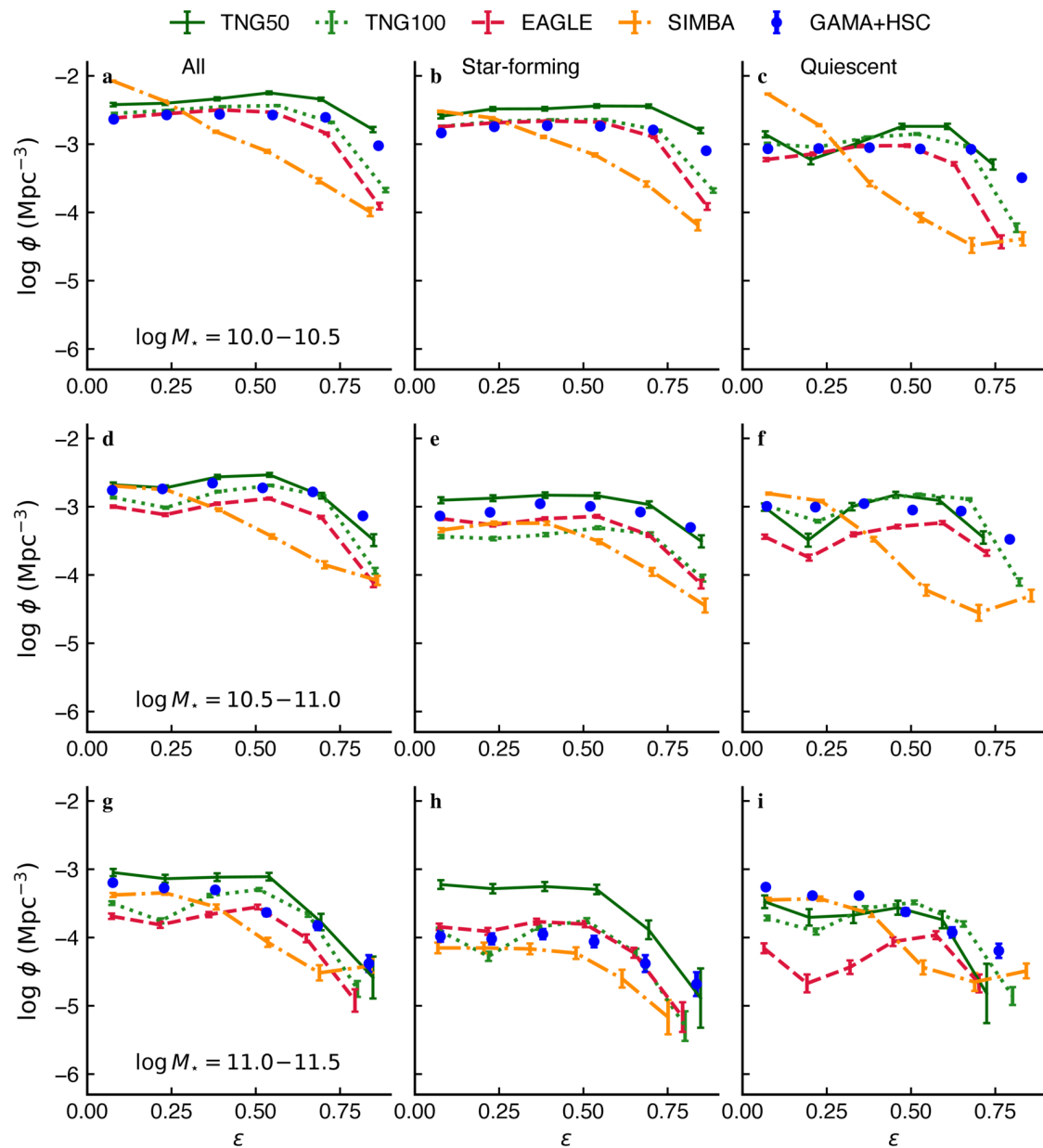
Figure 4. from Hassen M. Yesuf et al 2026 Astrophys. J. Lett. 1009 doi:10.3847/2041-8213/aea0c6 https://dx.doi.org/10.3847/2041-8213/aea0c6
