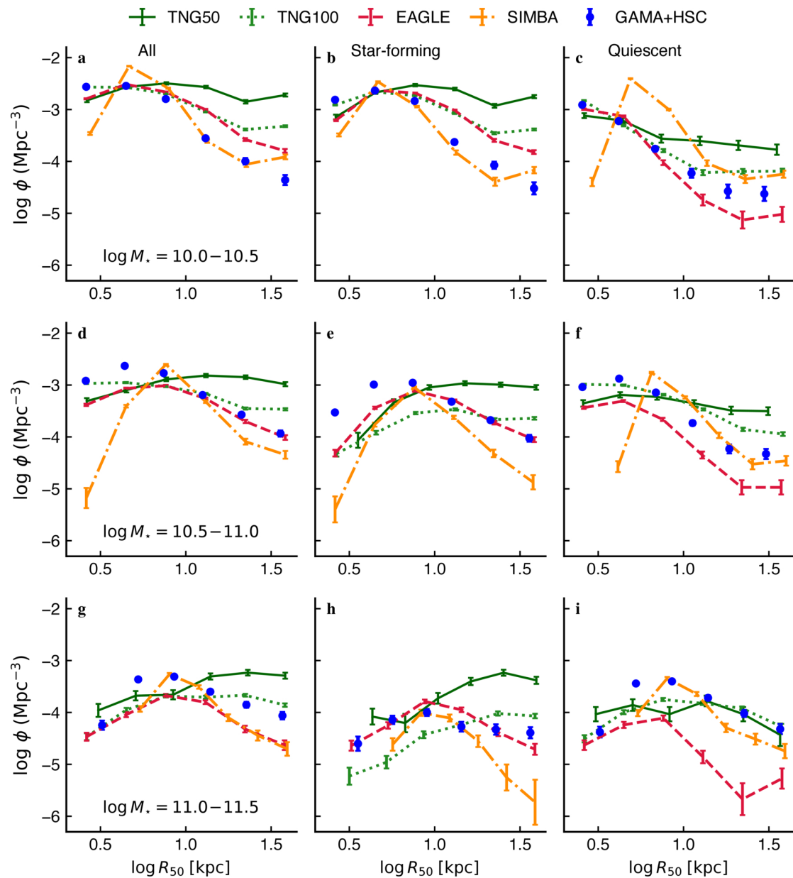
Figure 3. from Hassen M. Yesuf et al 2026 Astrophys. J. Lett. 1009 doi:10.3847/2041-8213/aea0c6 https://dx.doi.org/10.3847/2041-8213/aea0c6
