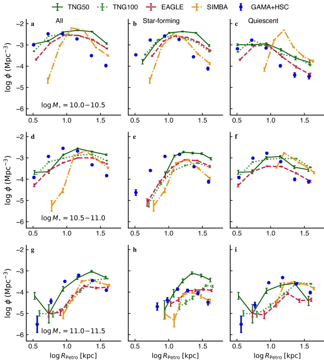
Figure 2. from Hassen M. Yesuf et al 2026 Astrophys. J. Lett. 1009 doi:10.3847/2041-8213/aea0c6 https://dx.doi.org/10.3847/2041-8213/aea0c6
