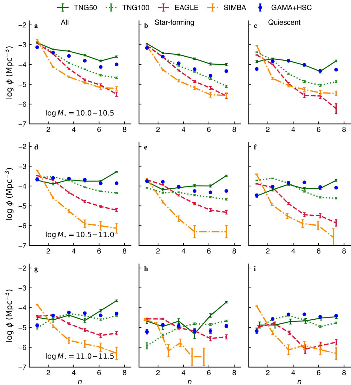
Figure 1. from Hassen M. Yesuf et al 2026 Astrophys. J. Lett. 1009 doi:10.3847/2041-8213/aea0c6 https://dx.doi.org/10.3847/2041-8213/aea0c6
