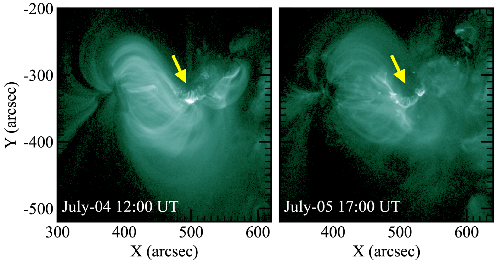
Figure 5. from Xinyue Wang et al 2026 Astrophys. J. Lett. 1010 doi:10.3847/2041-8213/aea099 https://dx.doi.org/10.3847/2041-8213/aea099 © 2026. The Author(s). Published by the American Astronomical Society.
