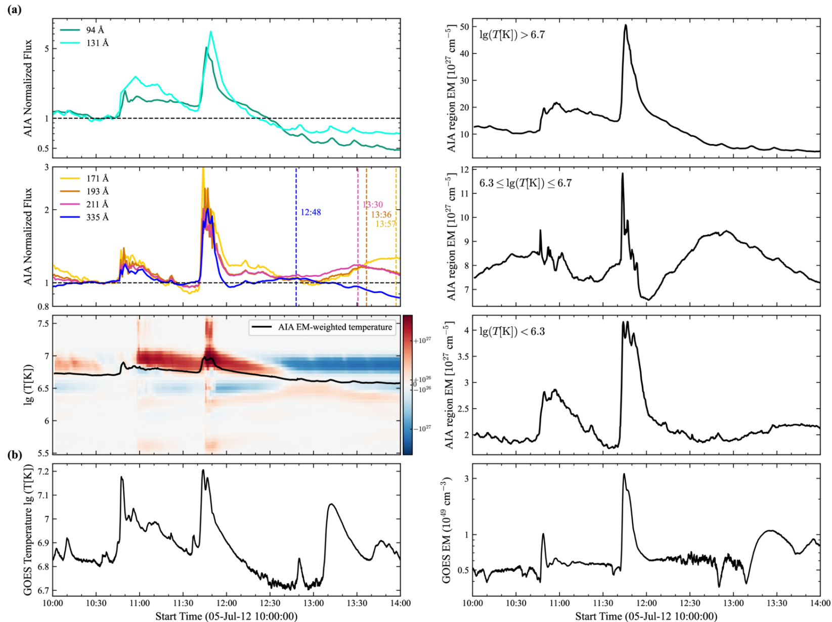
Figure 4. from Xinyue Wang et al 2026 Astrophys. J. Lett. 1010 doi:10.3847/2041-8213/aea099 https://dx.doi.org/10.3847/2041-8213/aea099 © 2026. The Author(s). Published by the American Astronomical Society.
