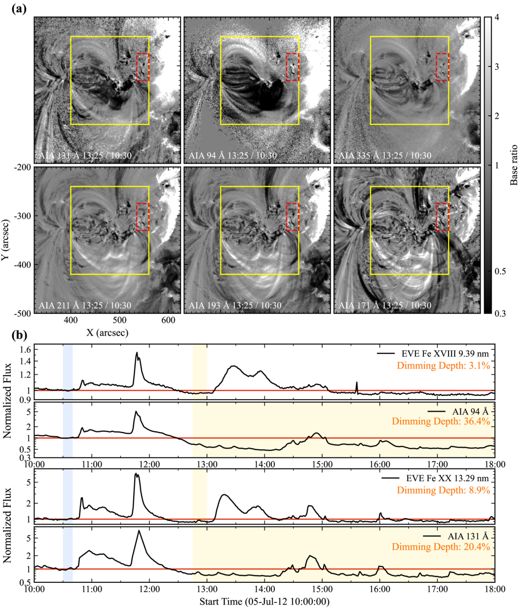
Figure 3. from Xinyue Wang et al 2026 Astrophys. J. Lett. 1010 doi:10.3847/2041-8213/aea099 https://dx.doi.org/10.3847/2041-8213/aea099 © 2026. The Author(s). Published by the American Astronomical Society.
