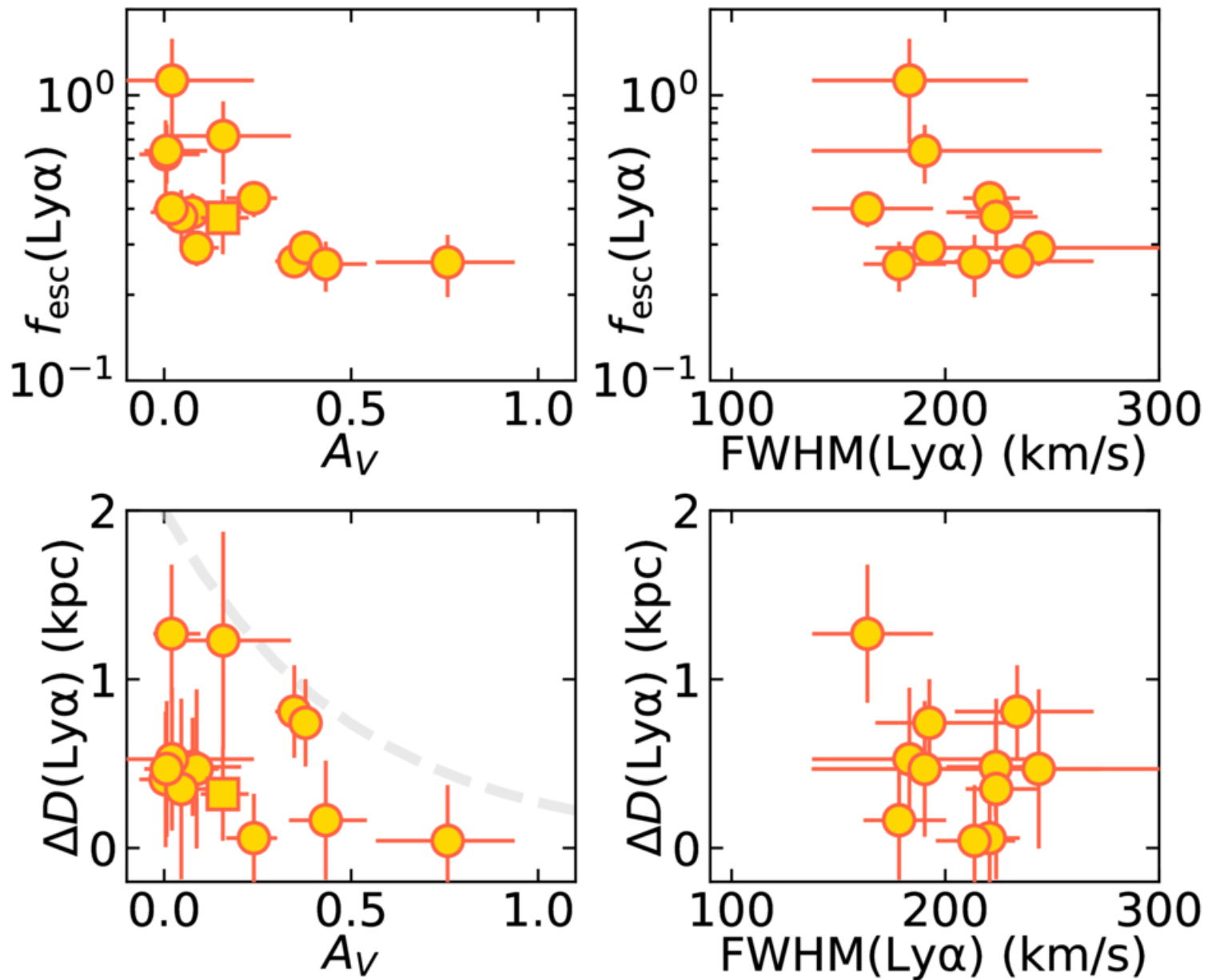
Figure 6. from Yuanhang Ning et al 2026 Astrophys. J. Lett. 1009 doi:10.3847/2041-8213/aea091 https://dx.doi.org/10.3847/2041-8213/aea091 © 2026. The Author(s). Published by the American Astronomical Society.
