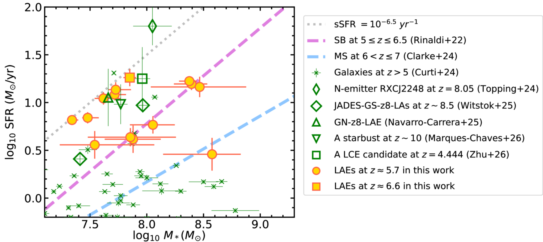
Figure 5. from Yuanhang Ning et al 2026 Astrophys. J. Lett. 1009 doi:10.3847/2041-8213/aea091 https://dx.doi.org/10.3847/2041-8213/aea091 © 2026. The Author(s). Published by the American Astronomical Society.
