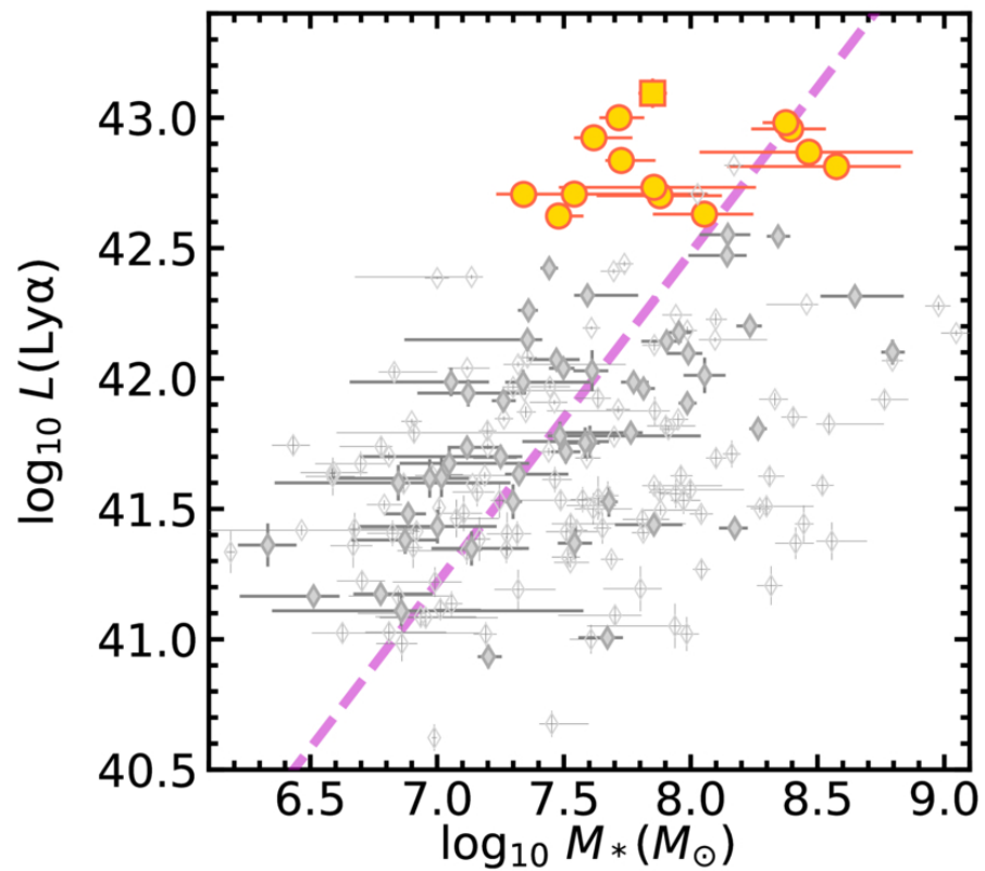
Figure 4. from Yuanhang Ning et al 2026 Astrophys. J. Lett. 1009 doi:10.3847/2041-8213/aea091 https://dx.doi.org/10.3847/2041-8213/aea091 © 2026. The Author(s). Published by the American Astronomical Society.
