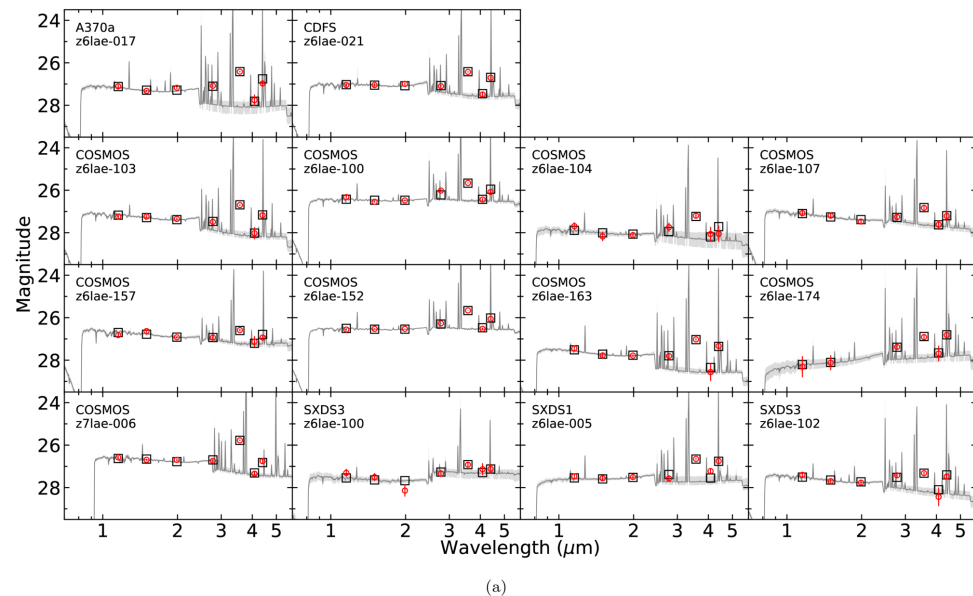
Figure 2. from Yuanhang Ning et al 2026 Astrophys. J. Lett. 1009 doi:10.3847/2041-8213/aea091 https://dx.doi.org/10.3847/2041-8213/aea091 © 2026. The Author(s). Published by the American Astronomical Society.
