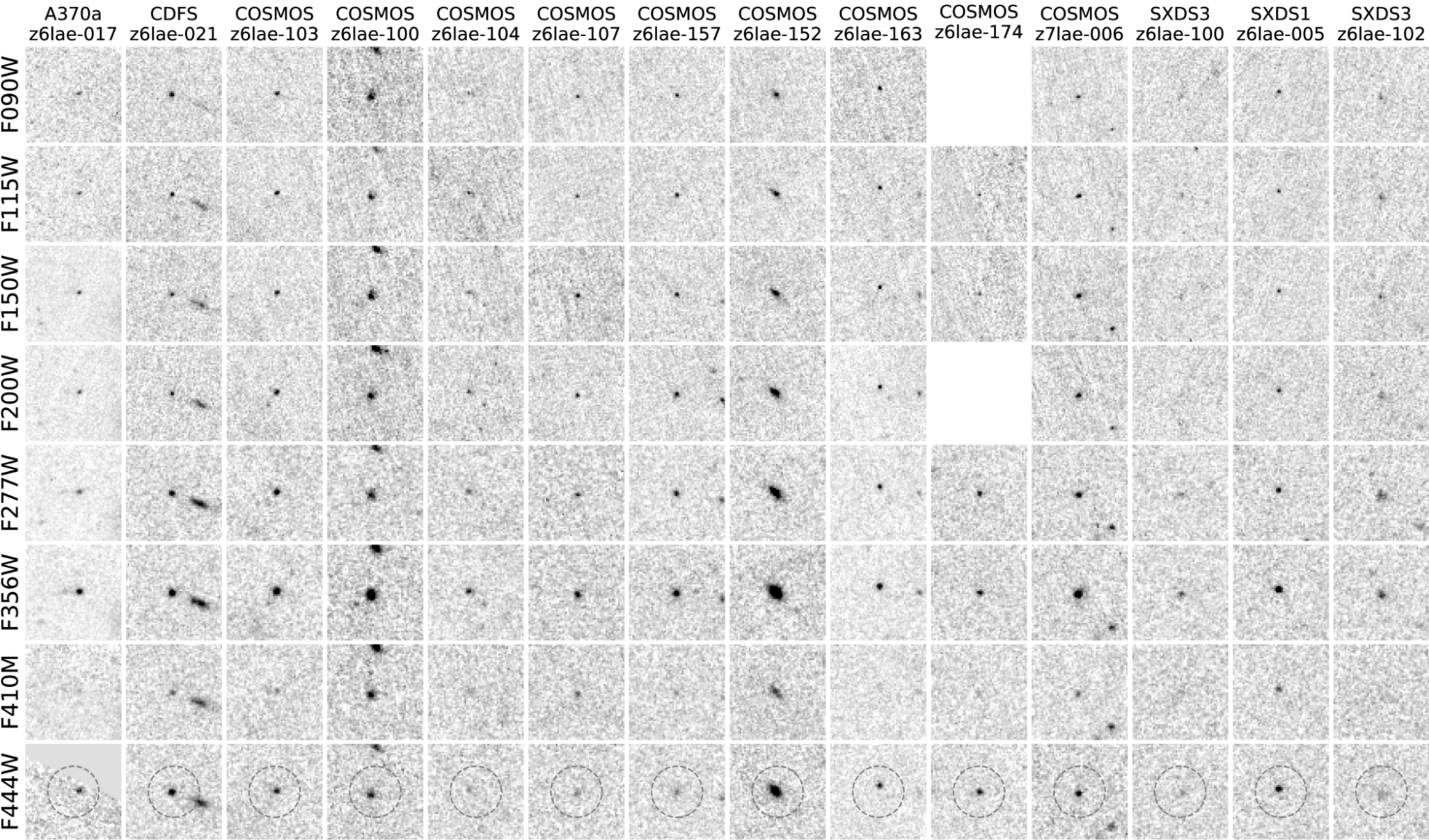
Figure 1. from Yuanhang Ning et al 2026 Astrophys. J. Lett. 1009 doi:10.3847/2041-8213/aea091 https://dx.doi.org/10.3847/2041-8213/aea091 © 2026. The Author(s). Published by the American Astronomical Society.
