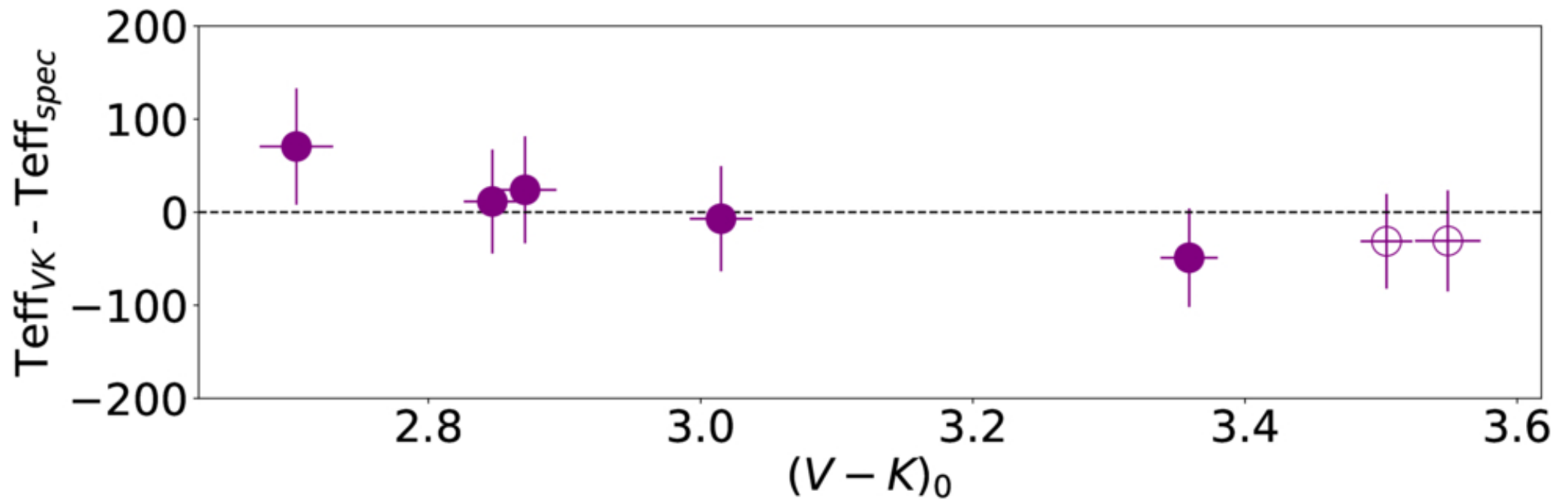
Figure C1. from Csilla Kalup et al 2026 Astrophys. J. Lett. 1009 doi:10.3847/2041-8213/aea08e https://dx.doi.org/10.3847/2041-8213/aea08e © 2026. The Author(s). Published by the American Astronomical Society.
