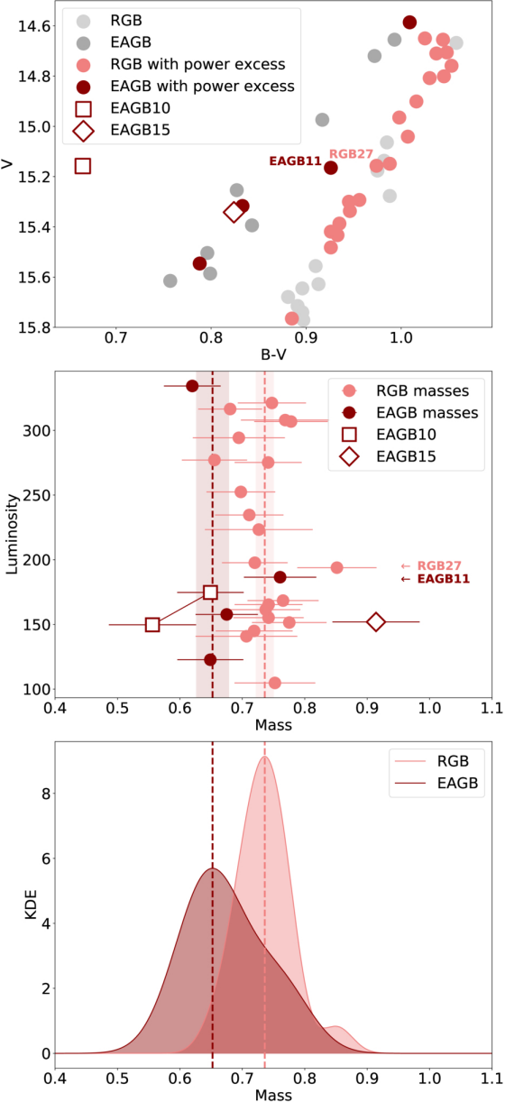
Figure 3. from Csilla Kalup et al 2026 Astrophys. J. Lett. 1009 doi:10.3847/2041-8213/aea08e https://dx.doi.org/10.3847/2041-8213/aea08e © 2026. The Author(s). Published by the American Astronomical Society.
