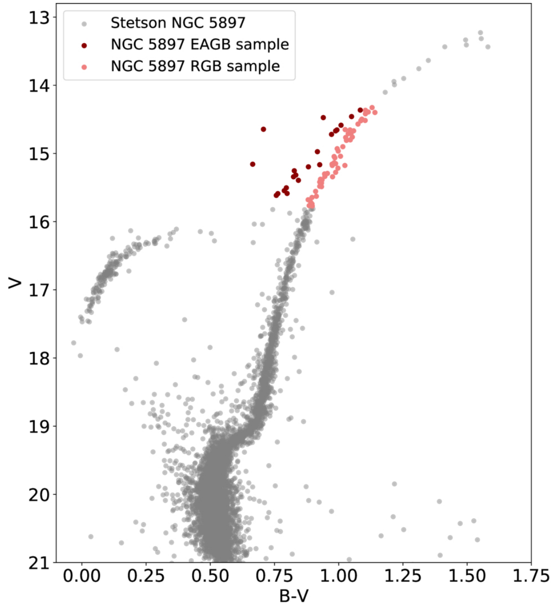
Figure 1. from Csilla Kalup et al 2026 Astrophys. J. Lett. 1009 doi:10.3847/2041-8213/aea08e https://dx.doi.org/10.3847/2041-8213/aea08e © 2026. The Author(s). Published by the American Astronomical Society.
