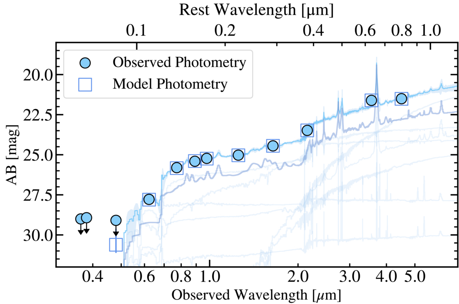
Figure B1. from Yilun Ma et al 2026 Astrophys. J. Lett. 1008 doi:10.3847/2041-8213/aea071 https://dx.doi.org/10.3847/2041-8213/aea071 © 2026. The Author(s). Published by the American Astronomical Society.
