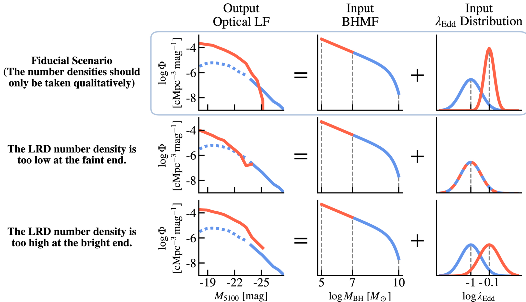
Figure 4. from Yilun Ma et al 2026 Astrophys. J. Lett. 1008 doi:10.3847/2041-8213/aea071 https://dx.doi.org/10.3847/2041-8213/aea071 © 2026. The Author(s). Published by the American Astronomical Society.
