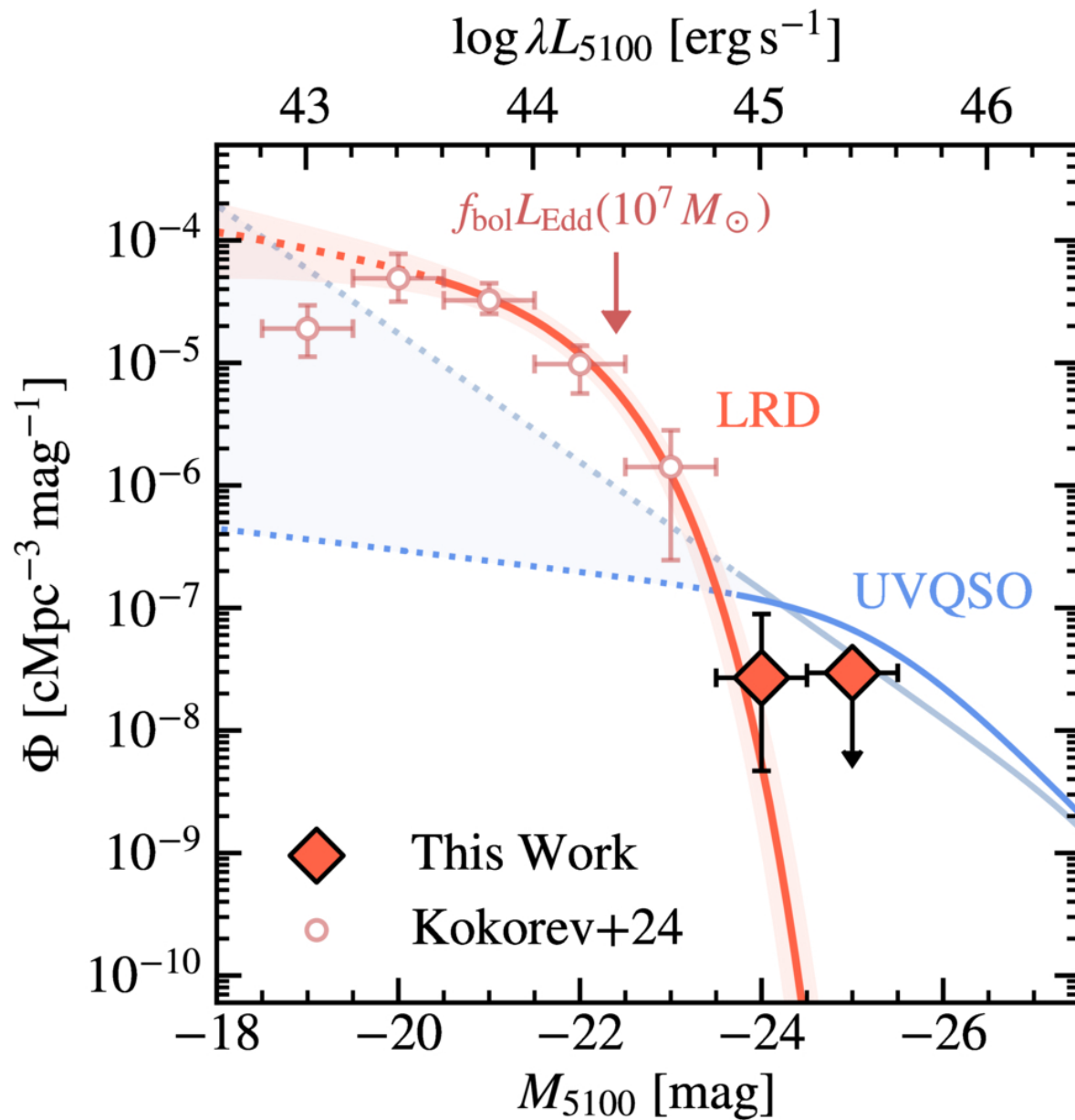
Figure 3. from Yilun Ma et al 2026 Astrophys. J. Lett. 1008 doi:10.3847/2041-8213/aea071 https://dx.doi.org/10.3847/2041-8213/aea071 © 2026. The Author(s). Published by the American Astronomical Society.
