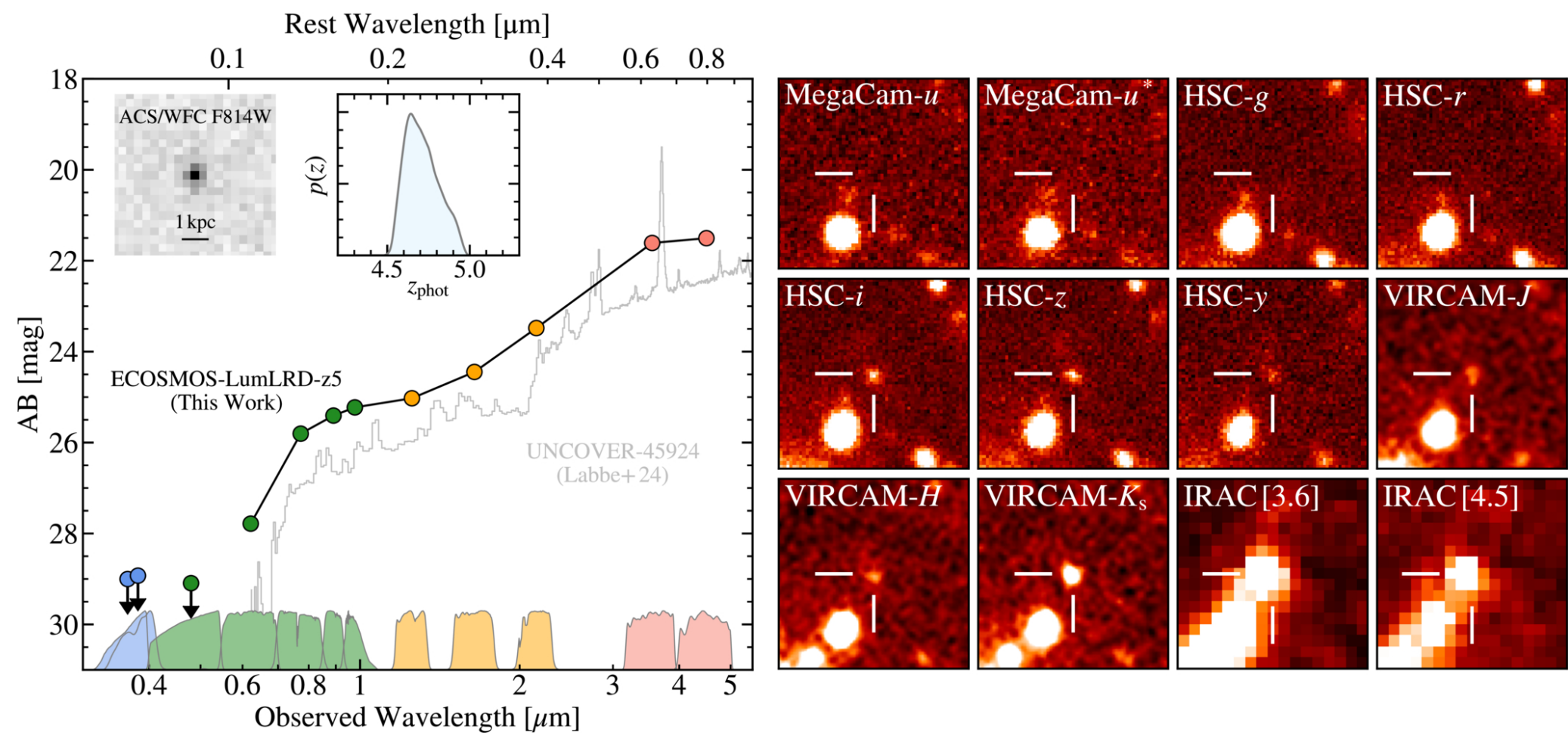
Figure 2. from Yilun Ma et al 2026 Astrophys. J. Lett. 1008 doi:10.3847/2041-8213/aea071 https://dx.doi.org/10.3847/2041-8213/aea071 © 2026. The Author(s). Published by the American Astronomical Society.
