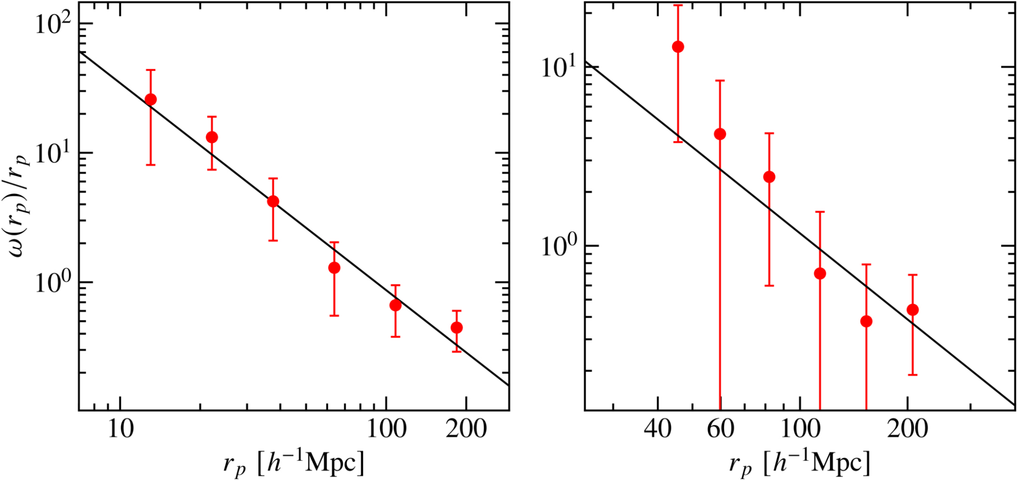
Figure 4. from Hao Meng et al 2026 Astrophys. J. Lett. 1009 doi:10.3847/2041-8213/aea06f https://dx.doi.org/10.3847/2041-8213/aea06f © 2026. The Author(s). Published by the American Astronomical Society.
