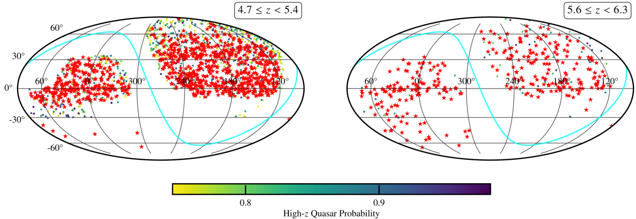
Figure 3. from Hao Meng et al 2026 Astrophys. J. Lett. 1009 doi:10.3847/2041-8213/aea06f https://dx.doi.org/10.3847/2041-8213/aea06f © 2026. The Author(s). Published by the American Astronomical Society.
