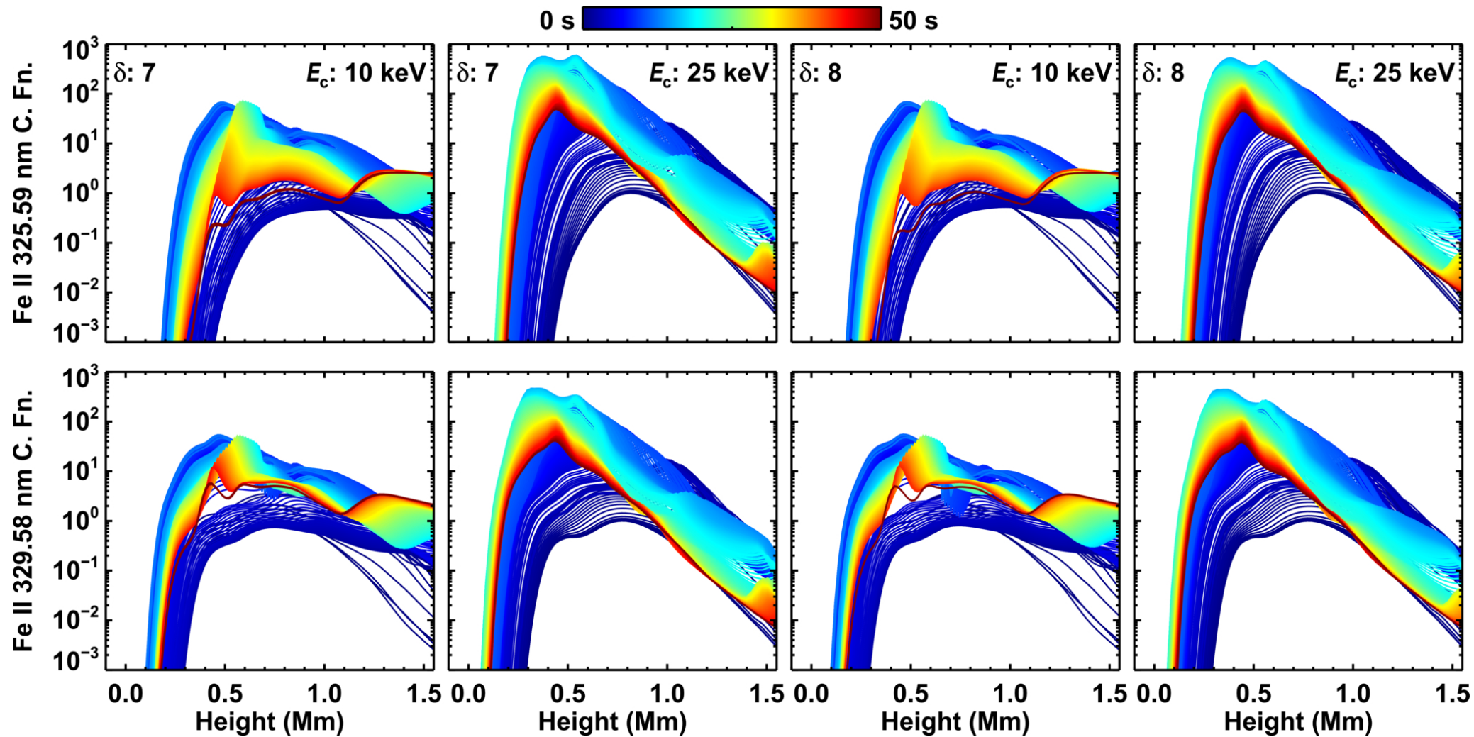
Figure B2. from L. P. Chitta et al 2026 Astrophys. J. Lett. 1008 doi:10.3847/2041-8213/aea06e https://dx.doi.org/10.3847/2041-8213/aea06e © 2026. The Author(s). Published by the American Astronomical Society.
