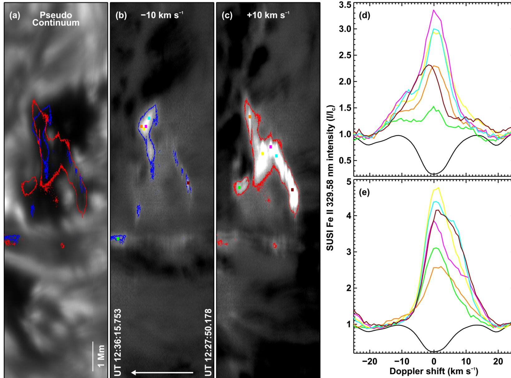
Figure 4. from L. P. Chitta et al 2026 Astrophys. J. Lett. 1008 doi:10.3847/2041-8213/aea06e https://dx.doi.org/10.3847/2041-8213/aea06e © 2026. The Author(s). Published by the American Astronomical Society.
