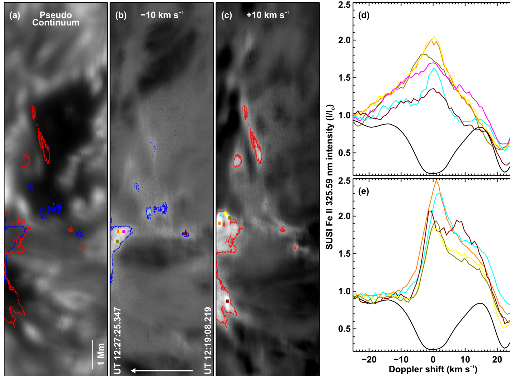
Figure 3. from L. P. Chitta et al 2026 Astrophys. J. Lett. 1008 doi:10.3847/2041-8213/aea06e https://dx.doi.org/10.3847/2041-8213/aea06e © 2026. The Author(s). Published by the American Astronomical Society.
