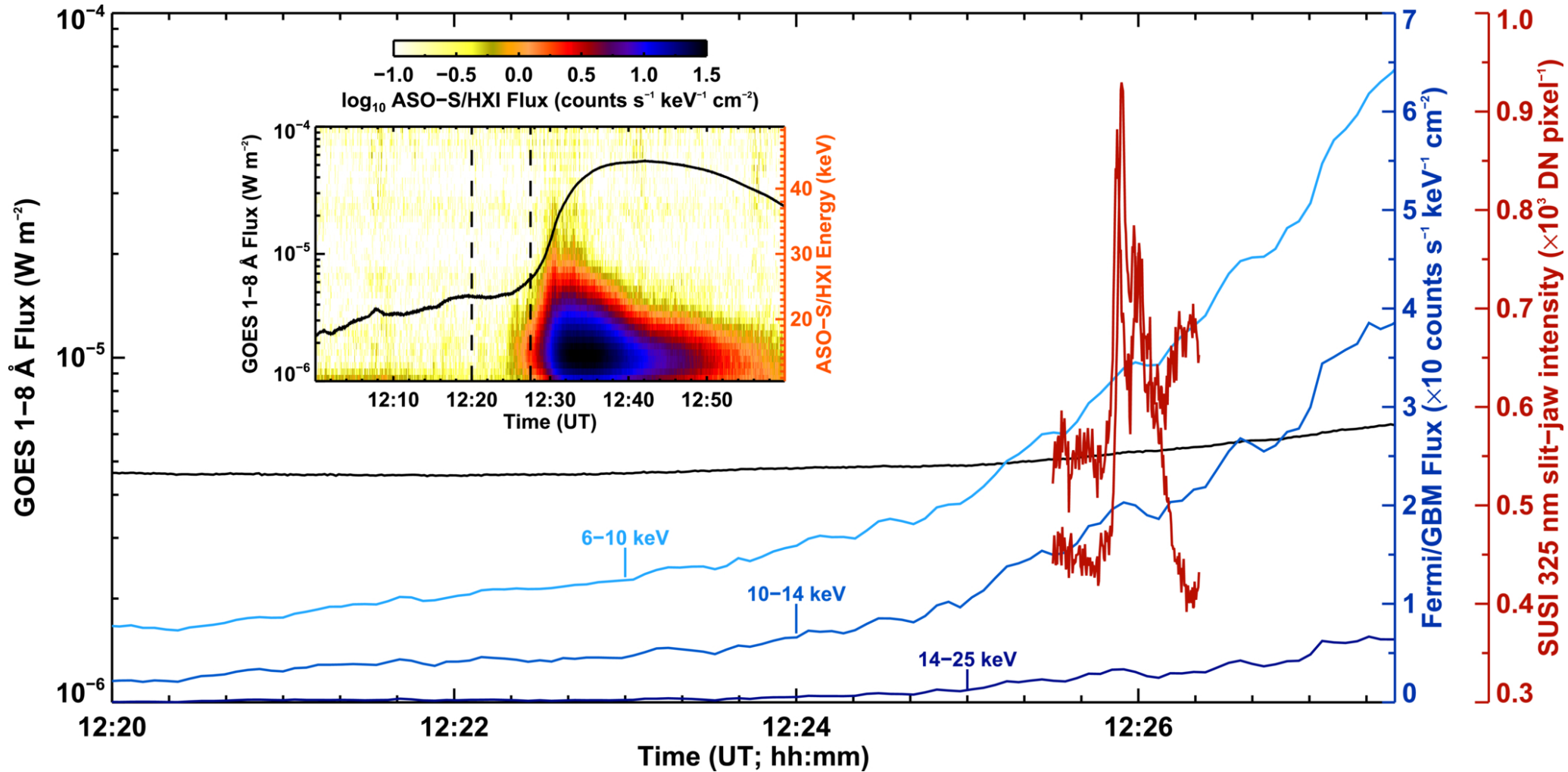
Figure 2. from L. P. Chitta et al 2026 Astrophys. J. Lett. 1008 doi:10.3847/2041-8213/aea06e https://dx.doi.org/10.3847/2041-8213/aea06e © 2026. The Author(s). Published by the American Astronomical Society.
