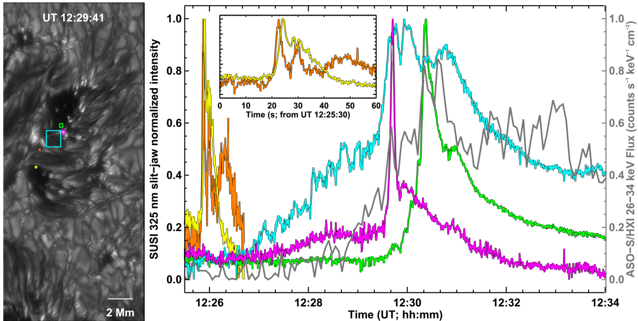
Figure 1. from L. P. Chitta et al 2026 Astrophys. J. Lett. 1008 doi:10.3847/2041-8213/aea06e https://dx.doi.org/10.3847/2041-8213/aea06e © 2026. The Author(s). Published by the American Astronomical Society.
