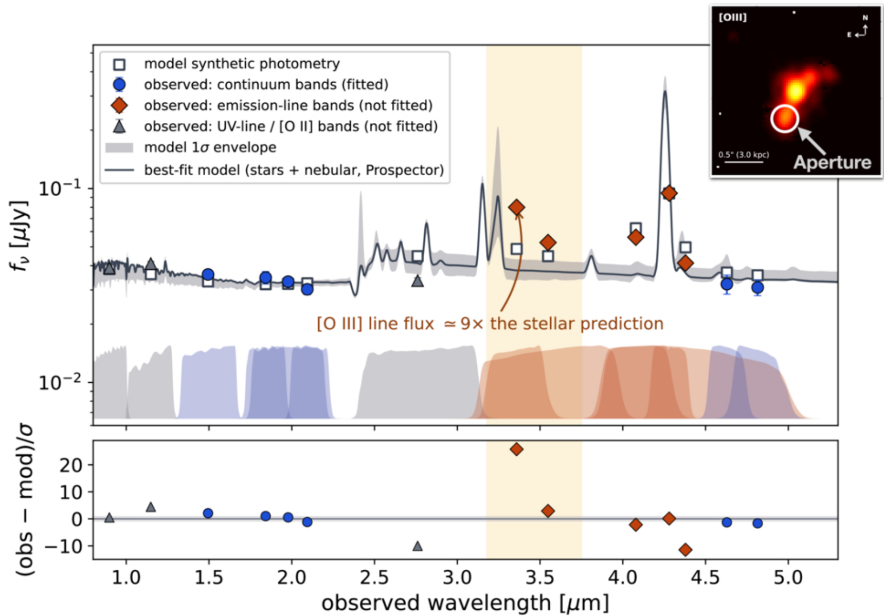
Figure 8. from Zhiyuan Ji et al 2026 Astrophys. J. Lett. 1008 doi:10.3847/2041-8213/ae9fea https://dx.doi.org/10.3847/2041-8213/ae9fea © 2026. The Author(s). Published by the American Astronomical Society.
