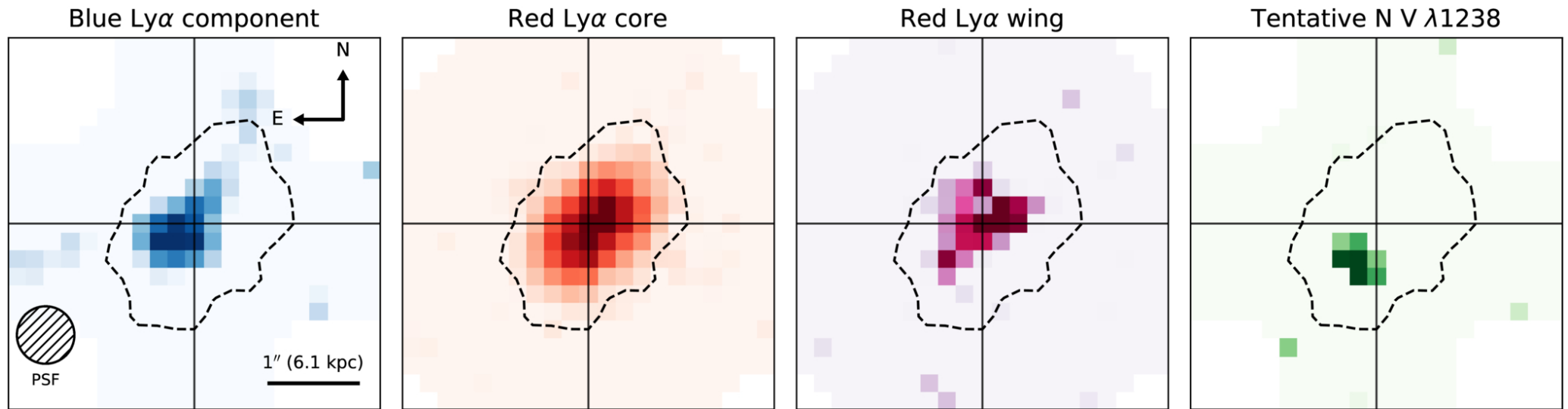
Figure 4. from Zhiyuan Ji et al 2026 Astrophys. J. Lett. 1008 doi:10.3847/2041-8213/ae9fea https://dx.doi.org/10.3847/2041-8213/ae9fea © 2026. The Author(s). Published by the American Astronomical Society.
