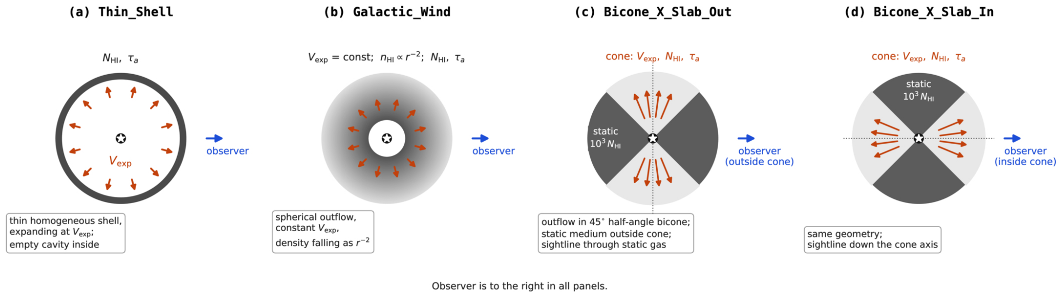
Figure 3. from Zhiyuan Ji et al 2026 Astrophys. J. Lett. 1008 doi:10.3847/2041-8213/ae9fea https://dx.doi.org/10.3847/2041-8213/ae9fea © 2026. The Author(s). Published by the American Astronomical Society.
