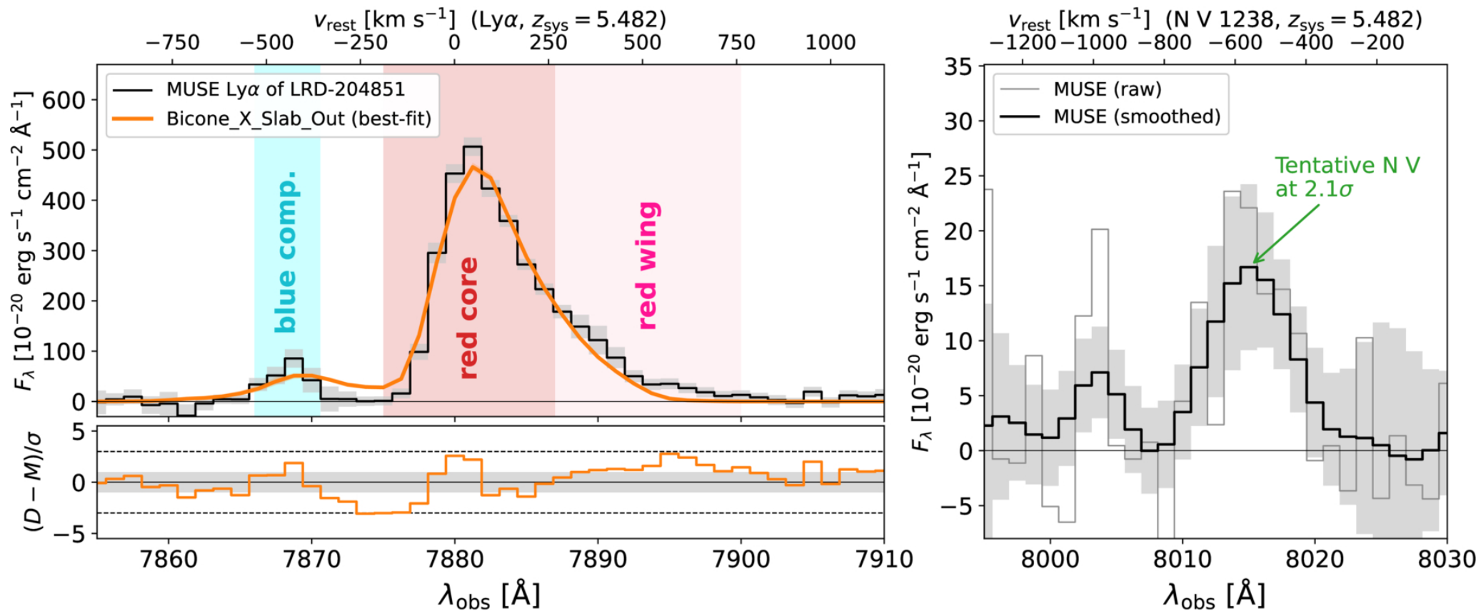
Figure 2. from Zhiyuan Ji et al 2026 Astrophys. J. Lett. 1008 doi:10.3847/2041-8213/ae9fea https://dx.doi.org/10.3847/2041-8213/ae9fea © 2026. The Author(s). Published by the American Astronomical Society.
