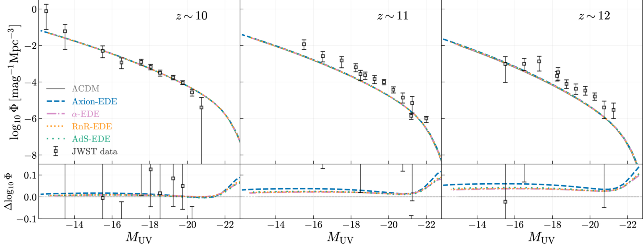
Figure 3. from Guo-Hong Du et al 2026 Astrophys. J. Lett. 1008 doi:10.3847/2041-8213/ae9f47 https://dx.doi.org/10.3847/2041-8213/ae9f47 © 2026. The Author(s). Published by the American Astronomical Society.
