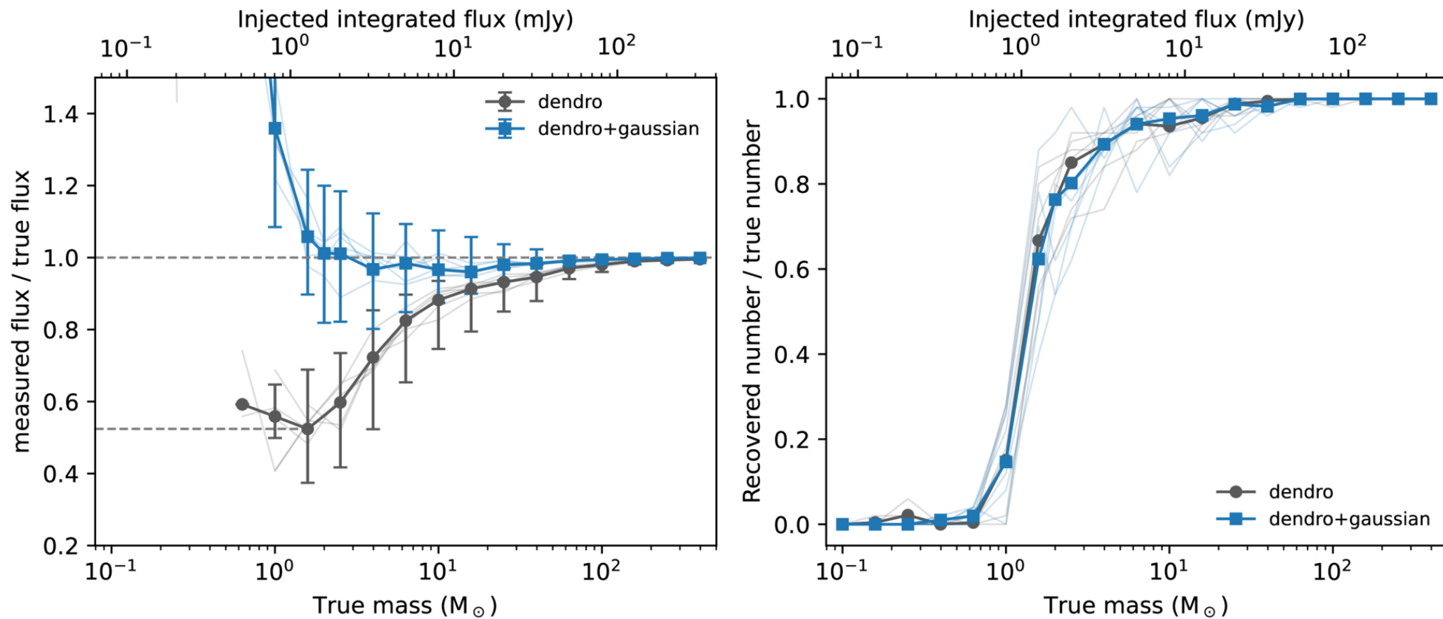
Figure C2. from Yu Cheng et al 2026 Astrophys. J. Lett. 1009 doi:10.3847/2041-8213/ae9f40 https://dx.doi.org/10.3847/2041-8213/ae9f40 © 2026. The Author(s). Published by the American Astronomical Society.
