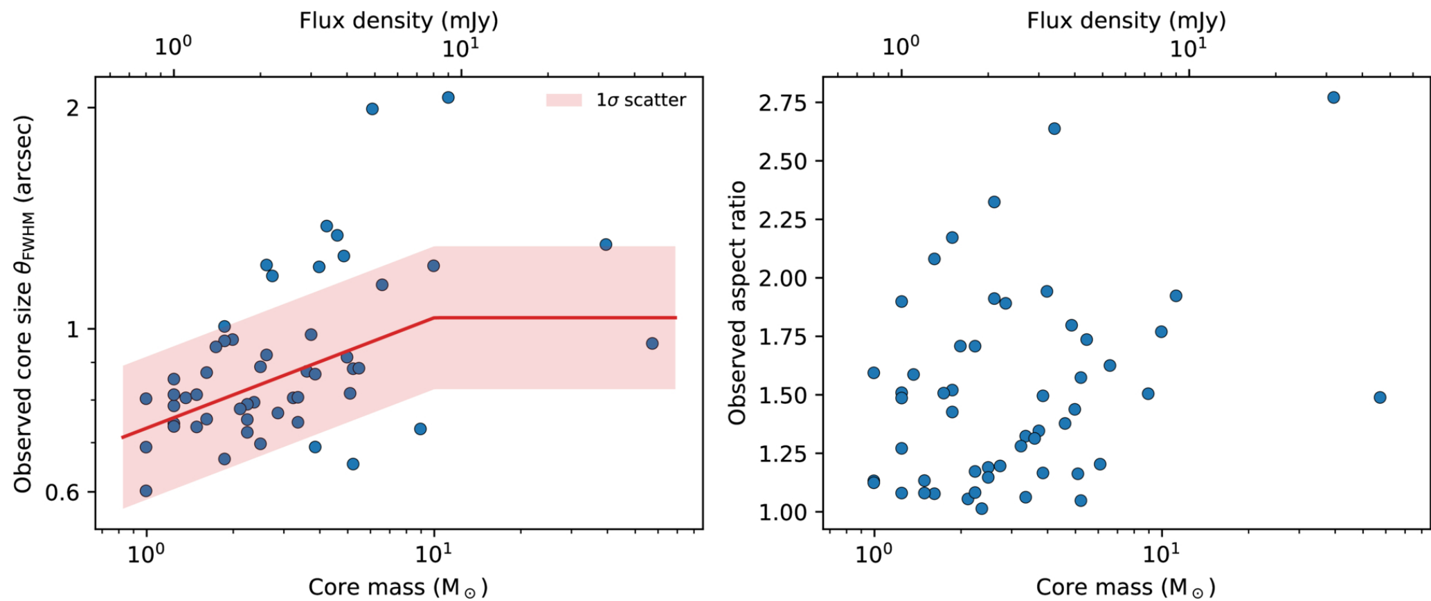
Figure C1. from Yu Cheng et al 2026 Astrophys. J. Lett. 1009 doi:10.3847/2041-8213/ae9f40 https://dx.doi.org/10.3847/2041-8213/ae9f40 © 2026. The Author(s). Published by the American Astronomical Society.
