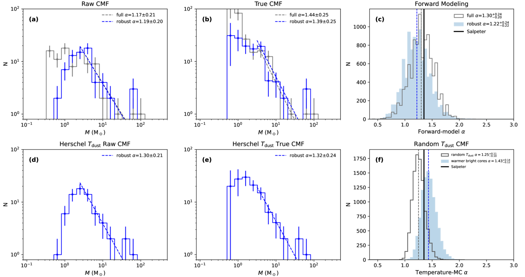
Figure 4. from Yu Cheng et al 2026 Astrophys. J. Lett. 1009 doi:10.3847/2041-8213/ae9f40 https://dx.doi.org/10.3847/2041-8213/ae9f40 © 2026. The Author(s). Published by the American Astronomical Society.
