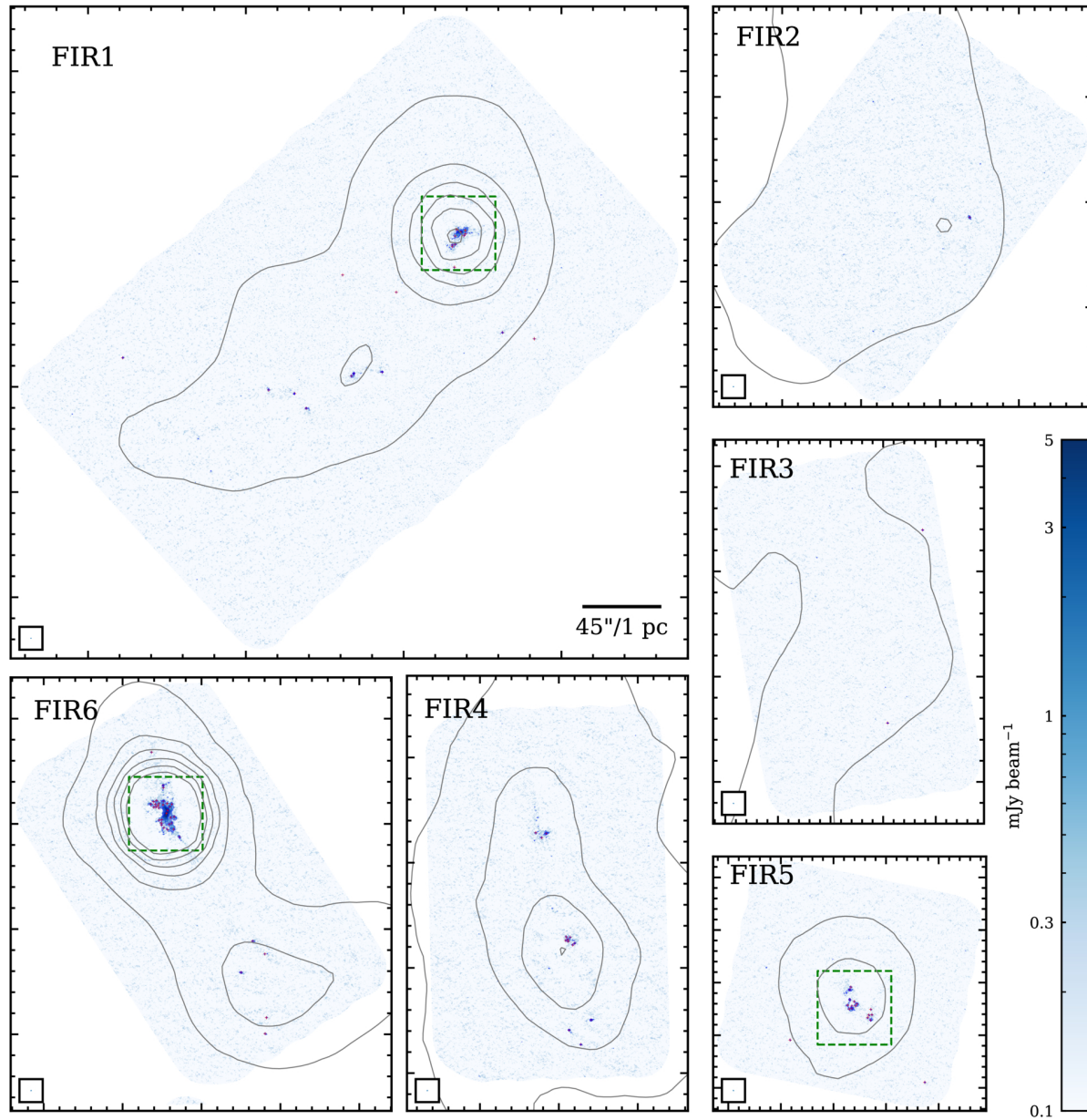
Figure 2. from Yu Cheng et al 2026 Astrophys. J. Lett. 1009 doi:10.3847/2041-8213/ae9f40 https://dx.doi.org/10.3847/2041-8213/ae9f40 © 2026. The Author(s). Published by the American Astronomical Society.
