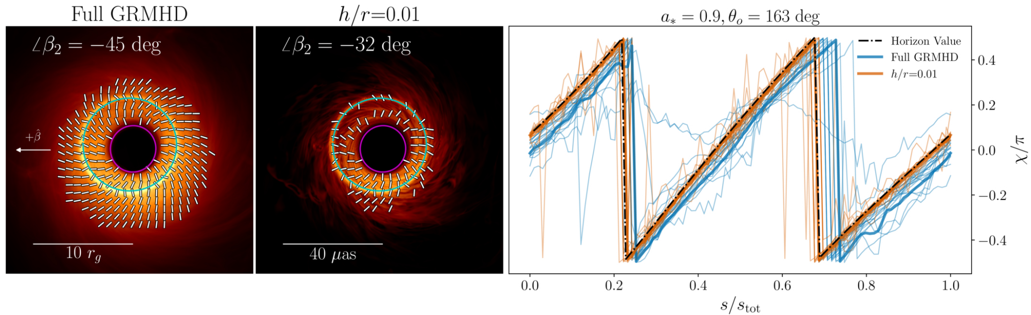
Figure 5. from Andrew Chael et al 2026 Astrophys. J. Lett. 1009 doi:10.3847/2041-8213/ae9ebf https://dx.doi.org/10.3847/2041-8213/ae9ebf © 2026. The Author(s). Published by the American Astronomical Society.
