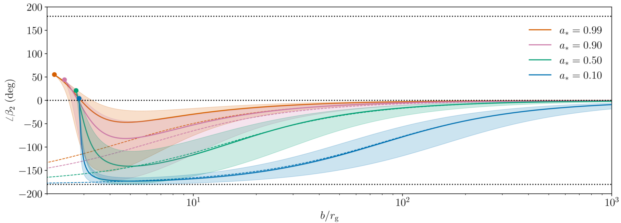
Figure 4. from Andrew Chael et al 2026 Astrophys. J. Lett. 1009 doi:10.3847/2041-8213/ae9ebf https://dx.doi.org/10.3847/2041-8213/ae9ebf © 2026. The Author(s). Published by the American Astronomical Society.
