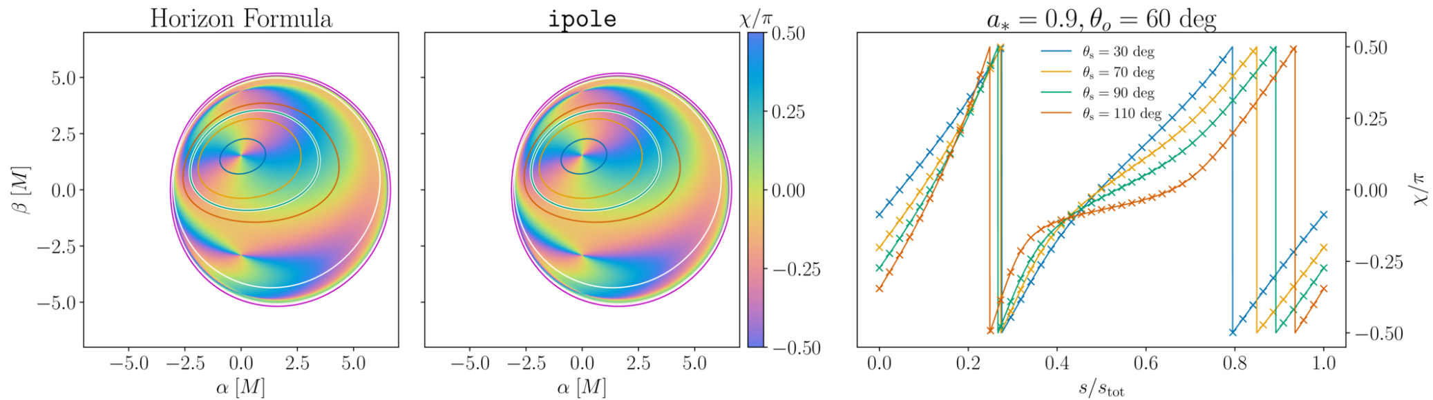
Figure 3. from Andrew Chael et al 2026 Astrophys. J. Lett. 1009 doi:10.3847/2041-8213/ae9ebf https://dx.doi.org/10.3847/2041-8213/ae9ebf © 2026. The Author(s). Published by the American Astronomical Society.
